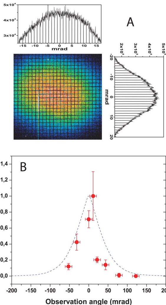
FIG. 9. (Color online). Angular distribution of the radiation for x-ray integrated energies beyond 1 keV. (a) Beam profile of the x-ray beam at n_e = 8 \times 10^{18} \text{ cm}^{-3} and the corresponding lineout graphics. (b) Angular distribution of the x-ray intensity for n_e = 1.1 \times 10^{19} \text{ cm}^{-3} (dotted line). The x-ray intensity has been normalized.
