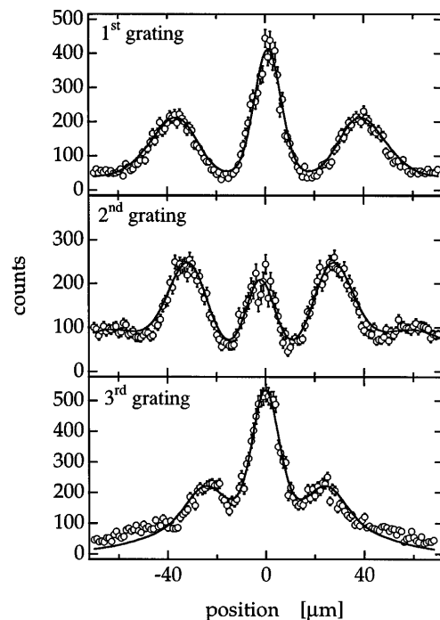
FIG. 3. Atom diffraction from the three standing light waves ( \lambda = 811 nm) used in the atom interferometer. The solid lines show a theoretical calculation including the various effects of the magnetic sublevel structure, of the velocity distribution and divergence of the atomic beam, and of spontaneous emission. The separation between the diffraction orders is best for the first grating, which has the farthest distance (1.25 m) from the detector.
