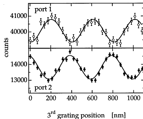
FIG. 2. Measured atom interference pattern for both output ports of the interferometer. The complementary intensity variations of the two output ports observed is a consequence of particle number conservation. The solid line is a fitted sinusoid.
