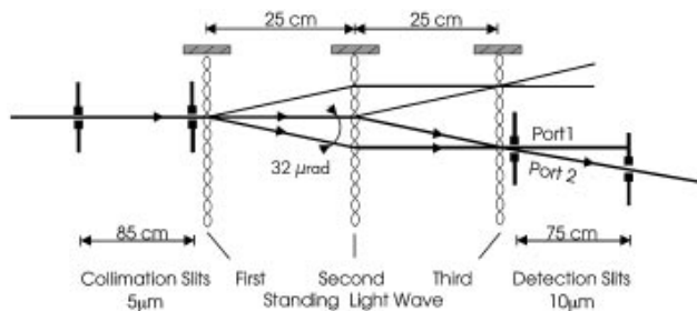
FIG. 1. Schematic arrangement of our interferometer setup (not to scale). The collimation slits for the incoming beam, the three standing light waves created by retroreflection at the mirrors, and the two final slits, one selecting a specific interferometer (thick lines) and the other selecting a specific output port are shown. For reasons of presentation, the wavelength of the light beams is greatly exaggerated. In the experiment the atomic beam was wide enough to cover more than 12 light wave antinodes.
