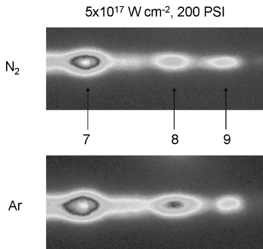
FIG. 5. Harmonic generation in high- Z gases. I=5\times 10^{17} W cm ^{-2} , n=10^{18} cm ^{-3} , and linear polarization.
